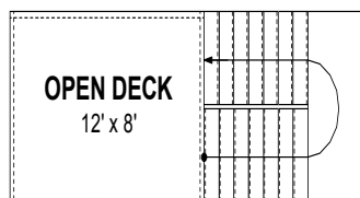
2ND FLOOR - FLOOR PLAN
